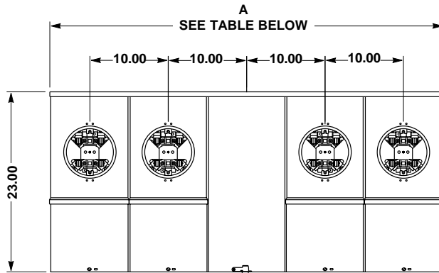
FRONT VIEW (244MCC)
