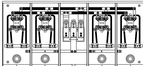
FRONT VIEW (W/OUT COVERS)
